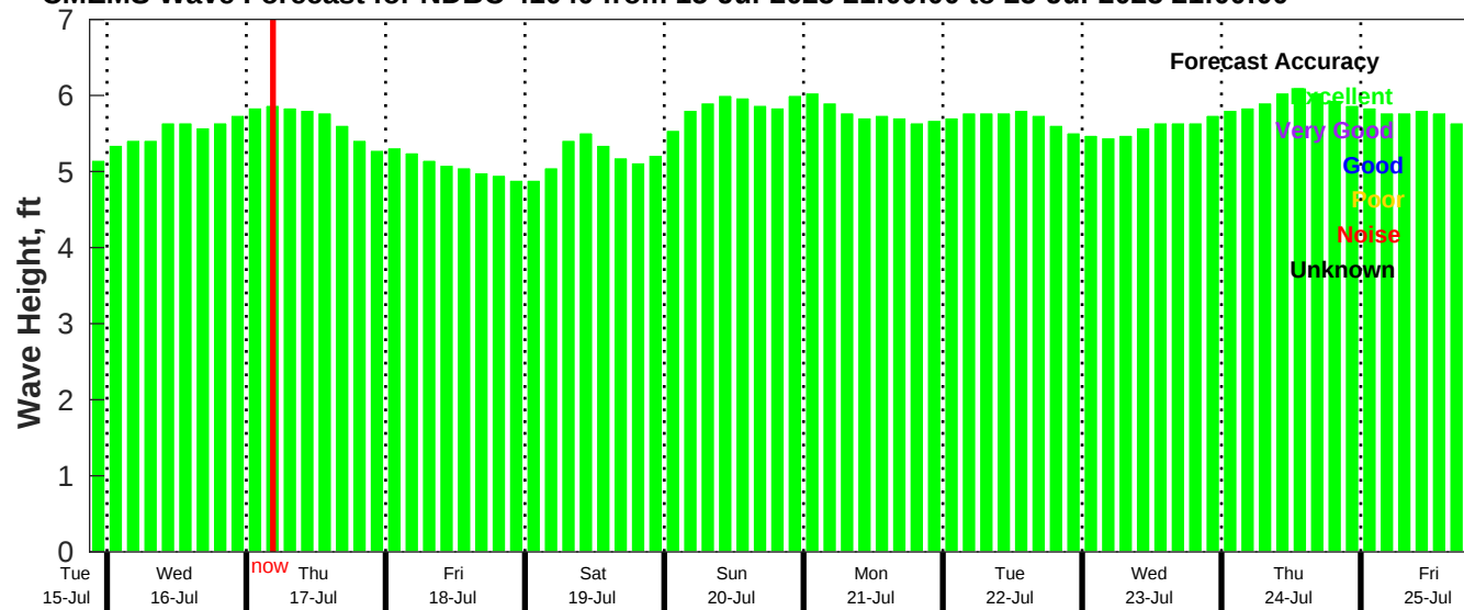
CMEMS Wave Forecast for NDBC 41040 from 15-Jul-2025 21:00:00 to 25-Jul-2025 21:00:00
