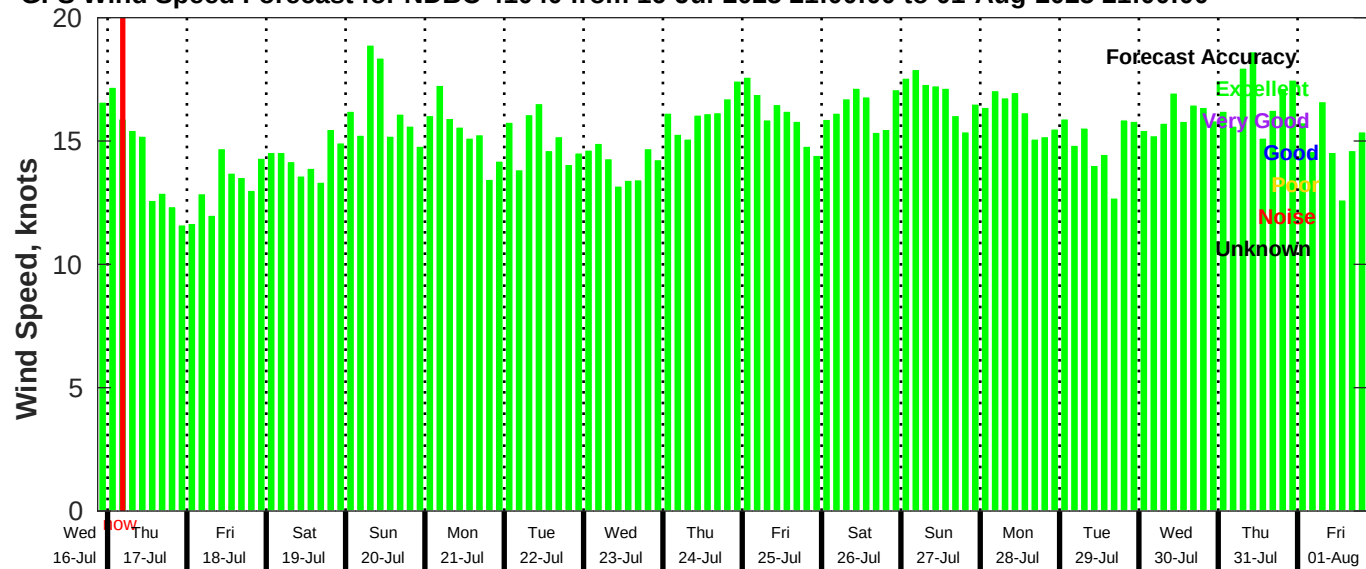
GFS Wind Speed Forecast for NDBC 41040 from 16-Jul-2025 21:00:00 to 01-Aug-2025 21:00:00
