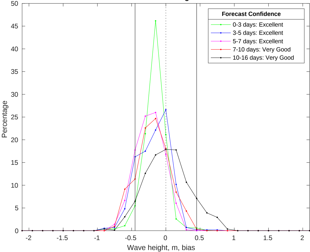
NDBC 42019 vs GFS Waves Bias Histogram: 17-Jul-2025
