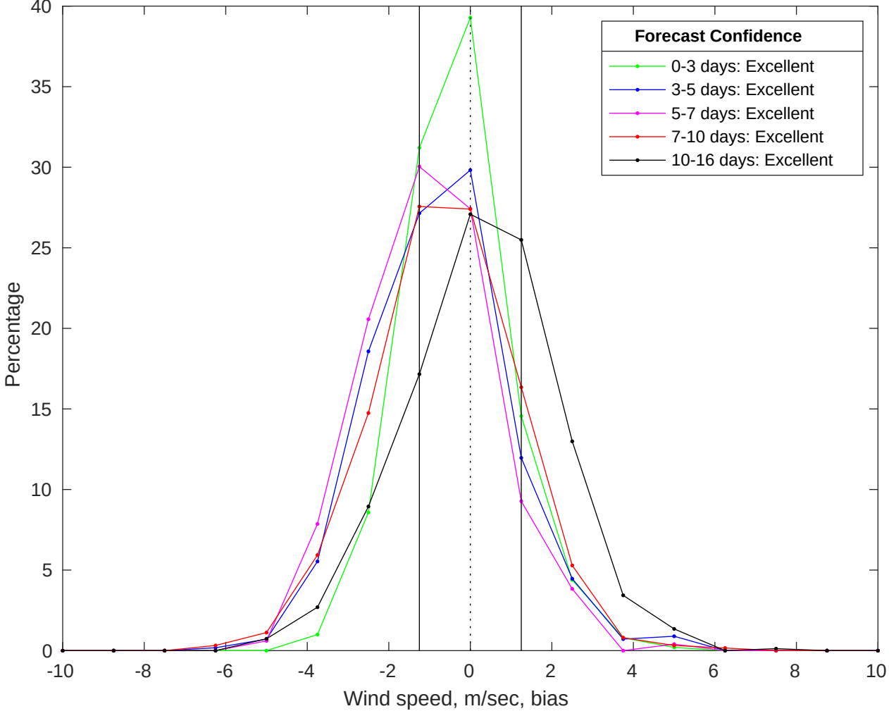
NDBC 42019 vs GFS Winds Bias Histogram: 17-Jul-2025
