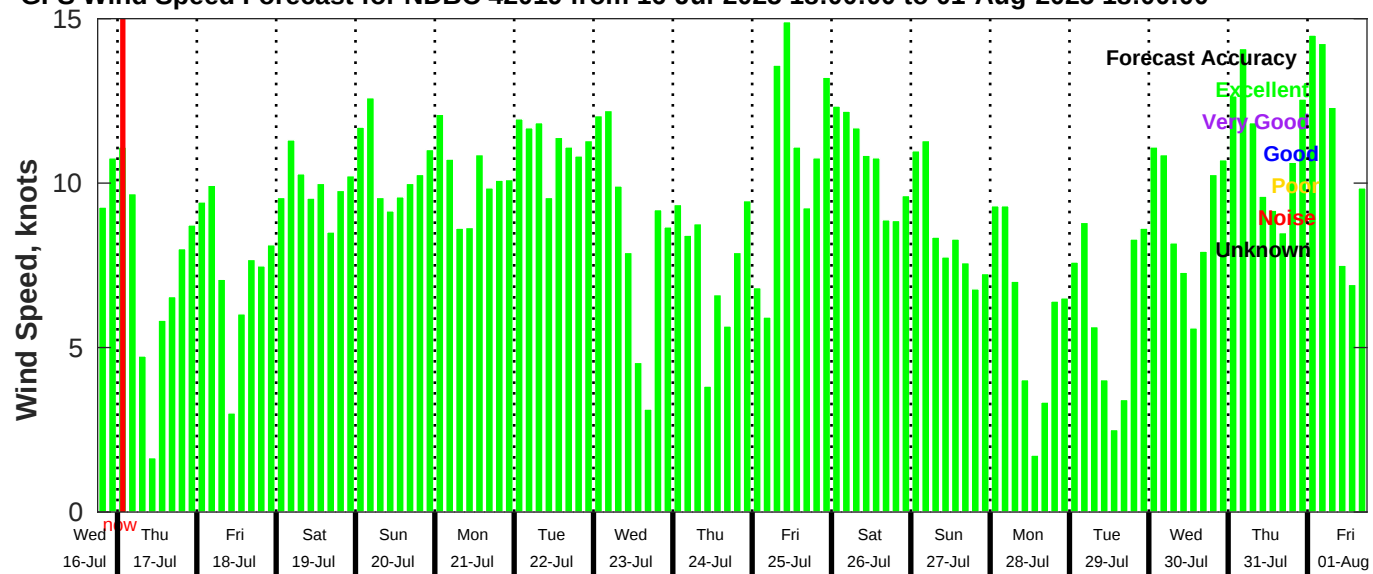
GFS Wind Speed Forecast for NDBC 42019 from 16-Jul-2025 18:00:00 to 01-Aug-2025 18:00:00
