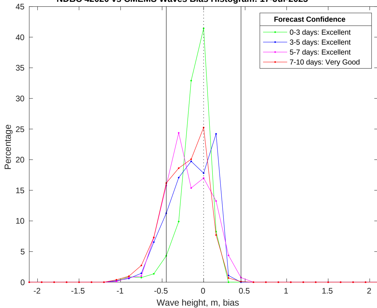
NDBC 42020 vs CMEMS Waves Bias Histogram: 17-Jul-2025
