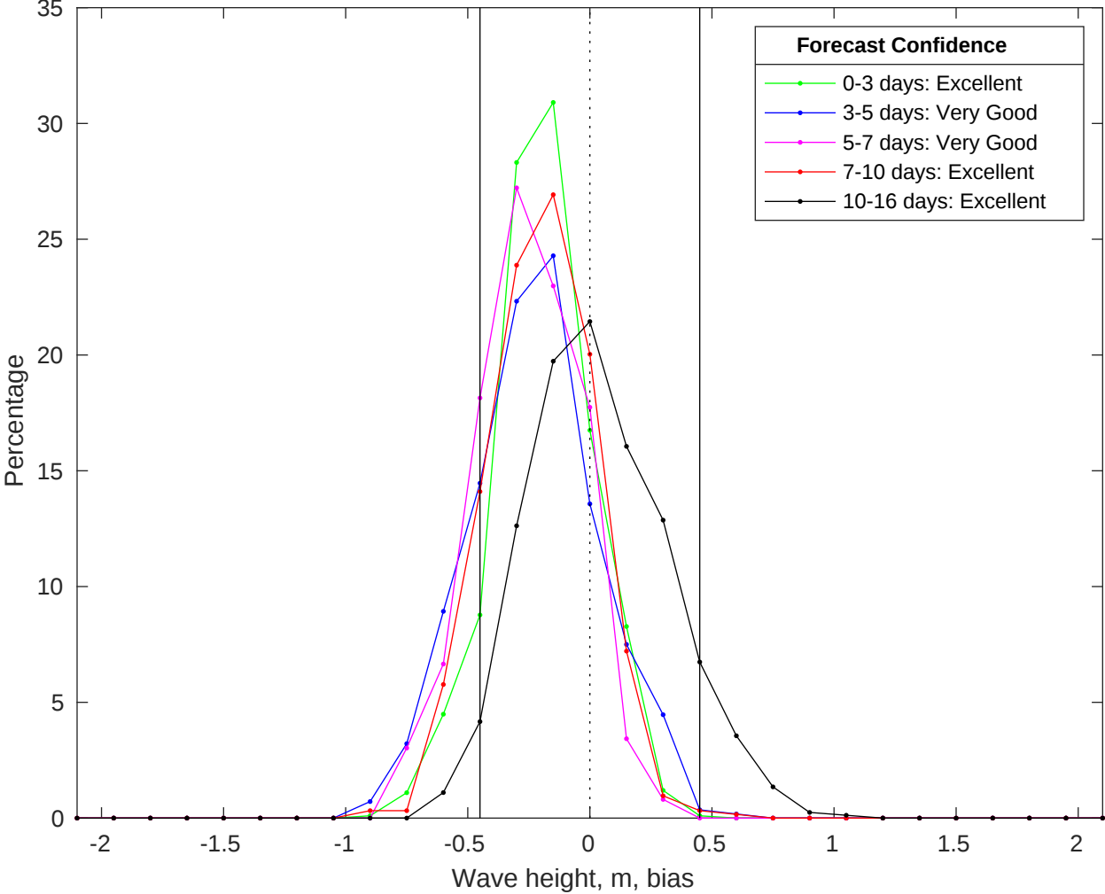
NDBC 42020 vs GFS Waves Bias Histogram: 17-Jul-2025
