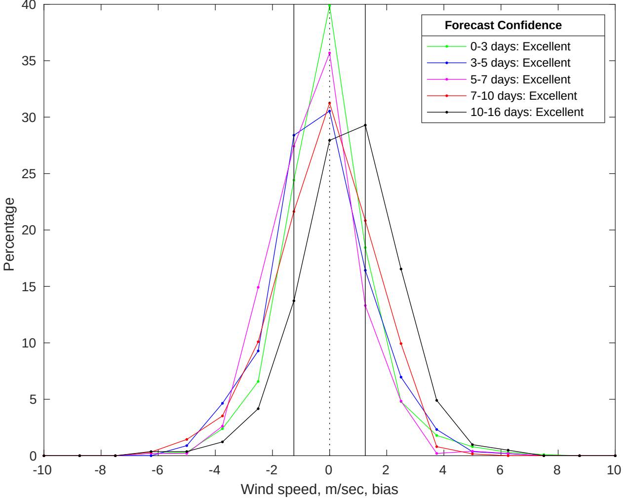
NDBC 42020 vs GFS Winds Bias Histogram: 17-Jul-2025
