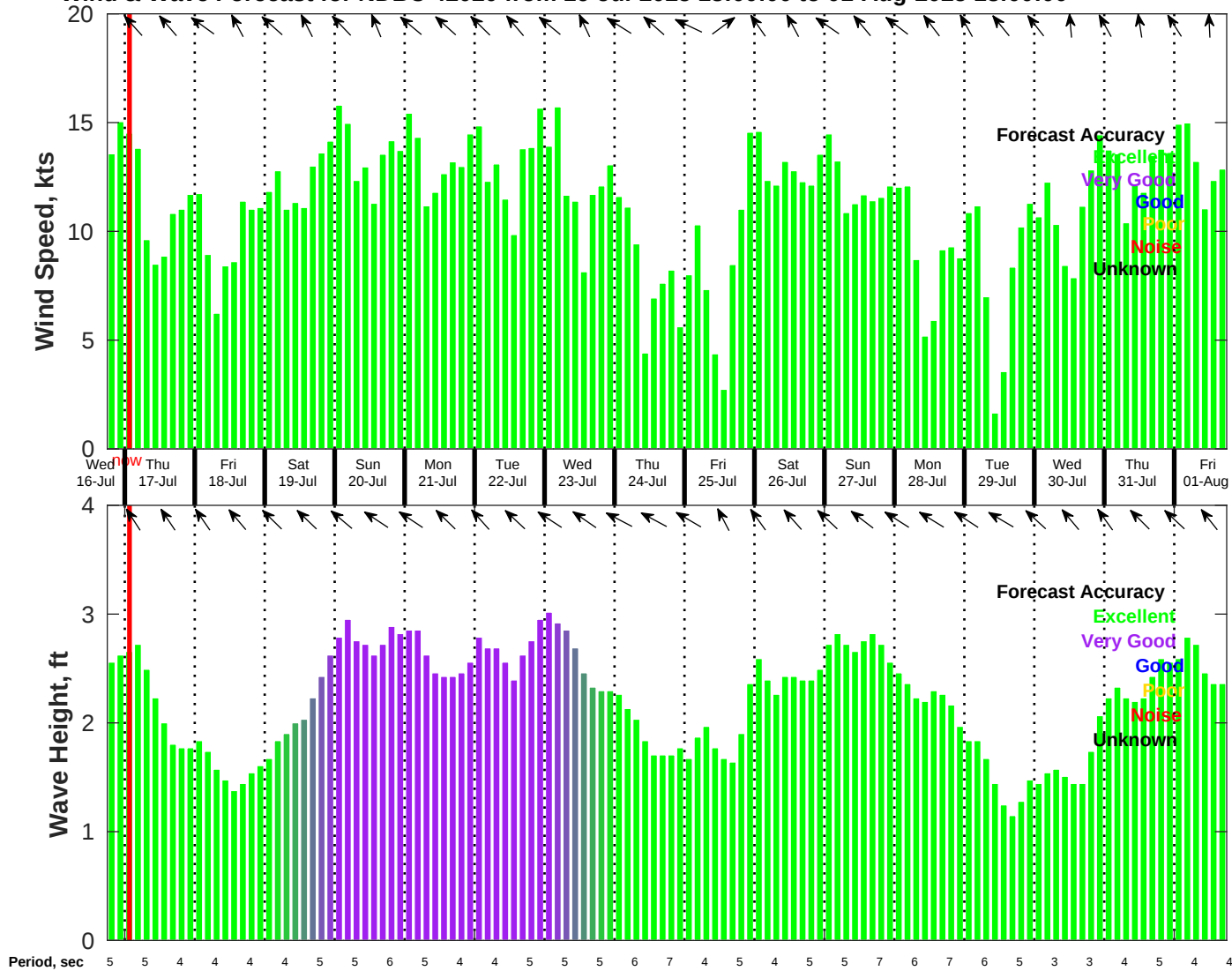
Wind & Wave Forecast for NDBC 42020 from 16-Jul-2025 18:00:00 to 01-Aug-2025 18:00:00
