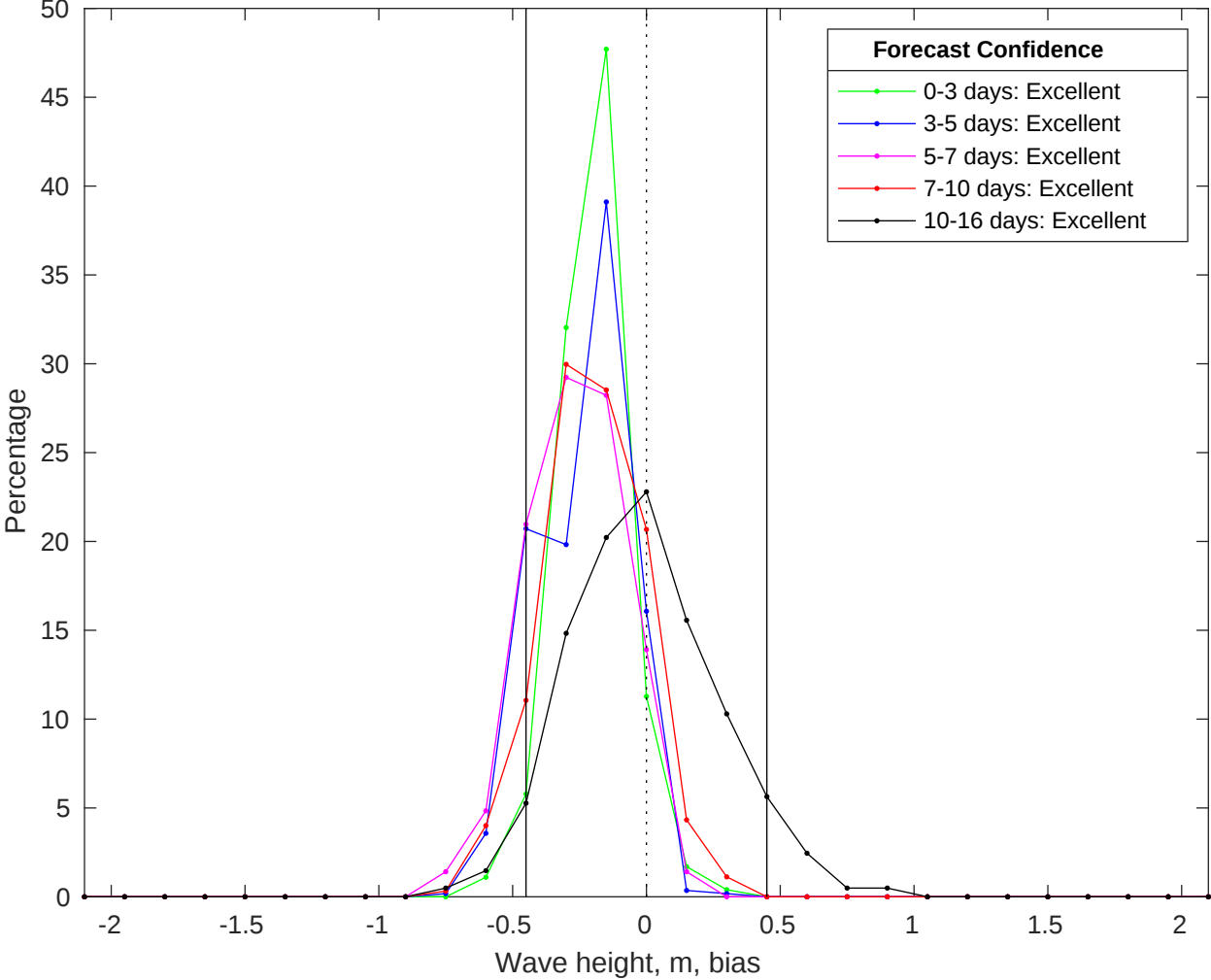
NDBC 42035 vs GFS Waves Bias Histogram: 17-Jul-2025
