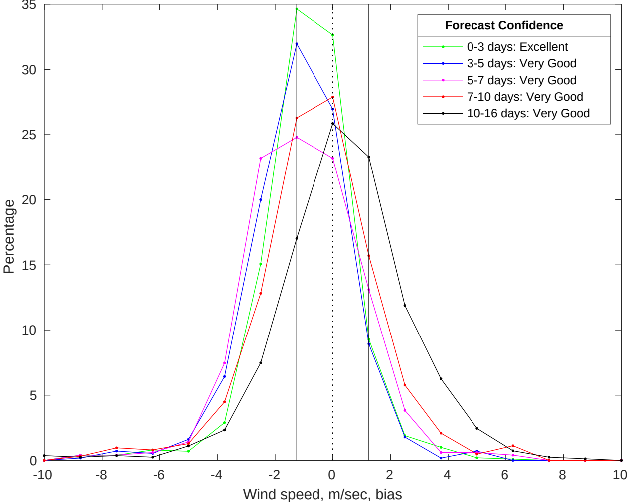
NDBC 42035 vs GFS Winds Bias Histogram: 17-Jul-2025
