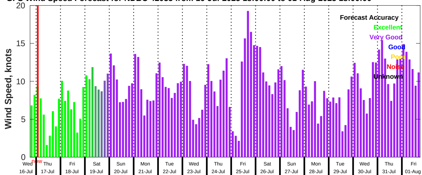
GFS Wind Speed Forecast for NDBC 42035 from 16-Jul-2025 18:00:00 to 01-Aug-2025 18:00:00
