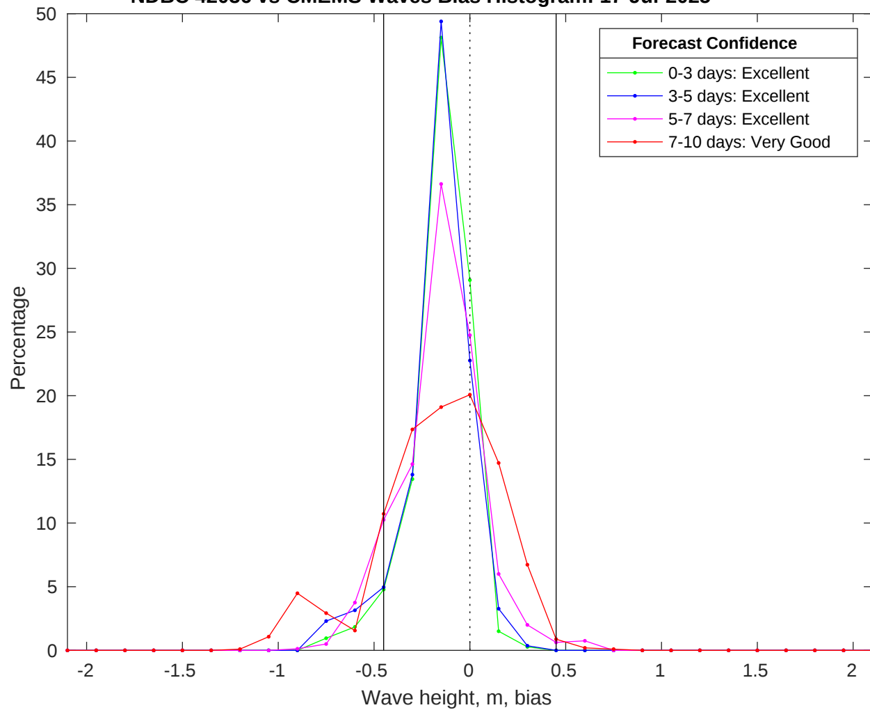
NDBC 42036 vs CMEMS Waves Bias Histogram: 17-Jul-2025
