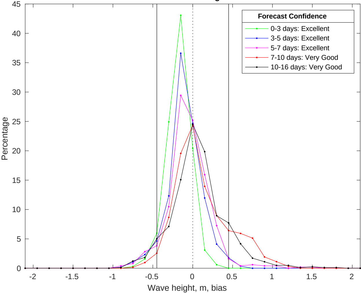
NDBC 42036 vs GFS Waves Bias Histogram: 17-Jul-2025
