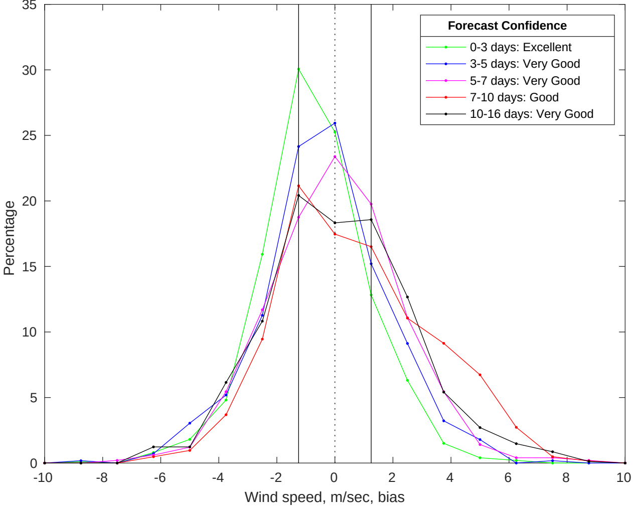
NDBC 42036 vs GFS Winds Bias Histogram: 17-Jul-2025
