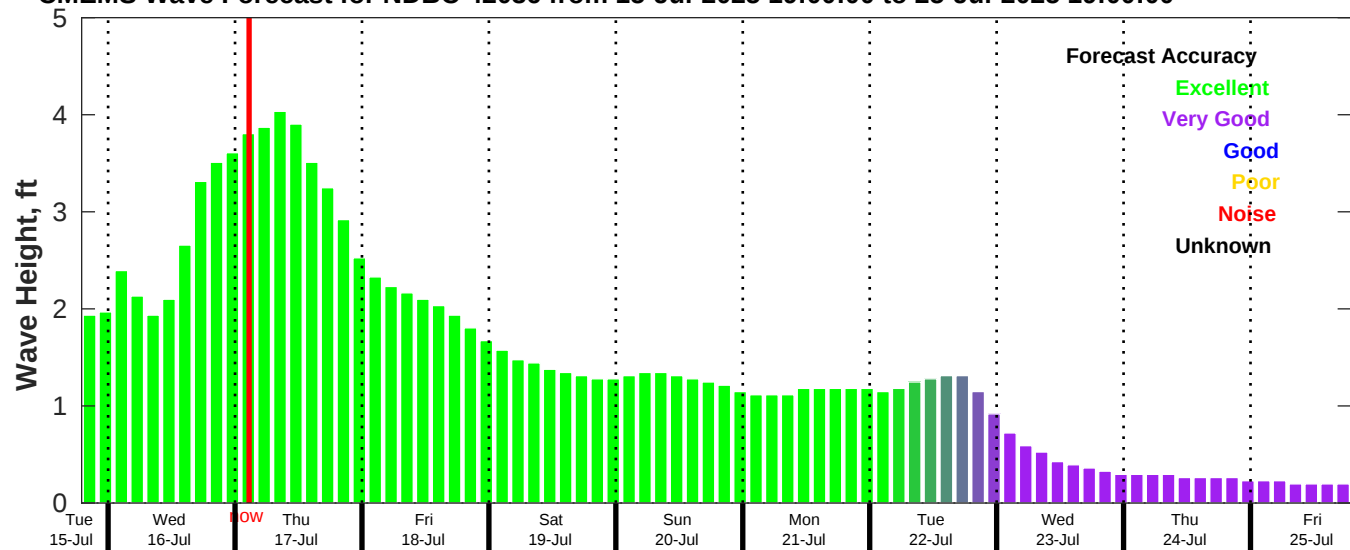
CMEMS Wave Forecast for NDBC 42036 from 15-Jul-2025 19:00:00 to 25-Jul-2025 19:00:00
