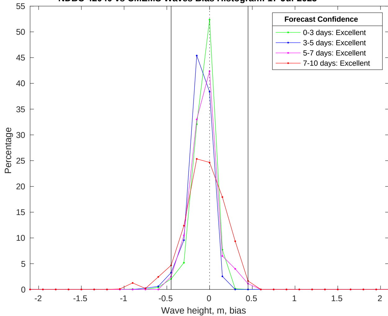
NDBC 42040 vs CMEMS Waves Bias Histogram: 17-Jul-2025
