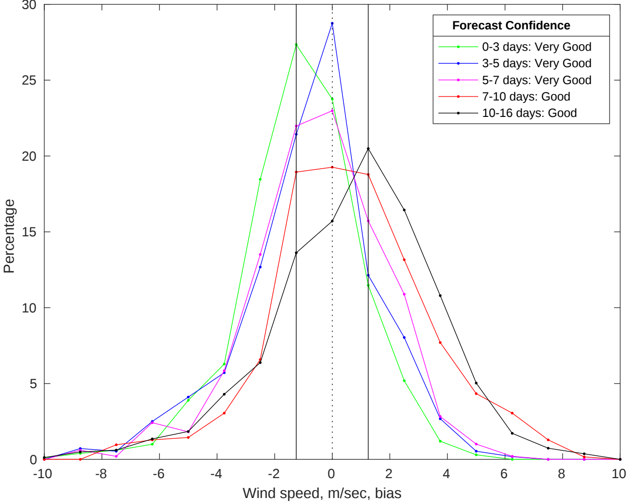
NDBC 42040 vs GFS Winds Bias Histogram: 17-Jul-2025
