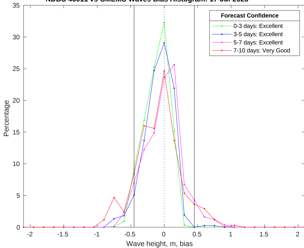
NDBC 46011 vs CMEMS Waves Bias Histogram: 17-Jul-2025
