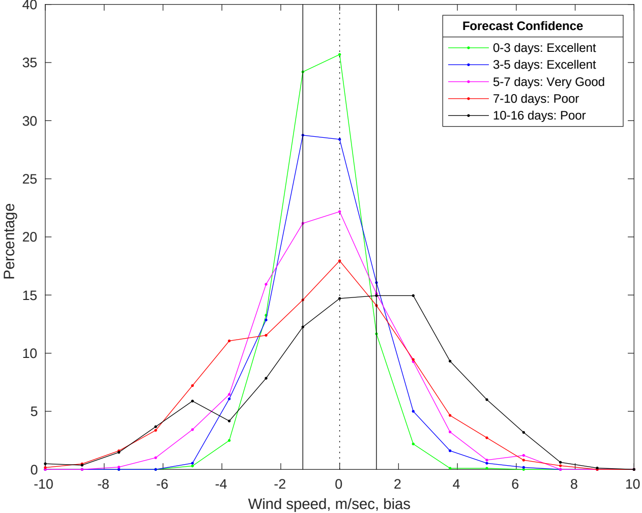
NDBC 46011 vs GFS Winds Bias Histogram: 17-Jul-2025
