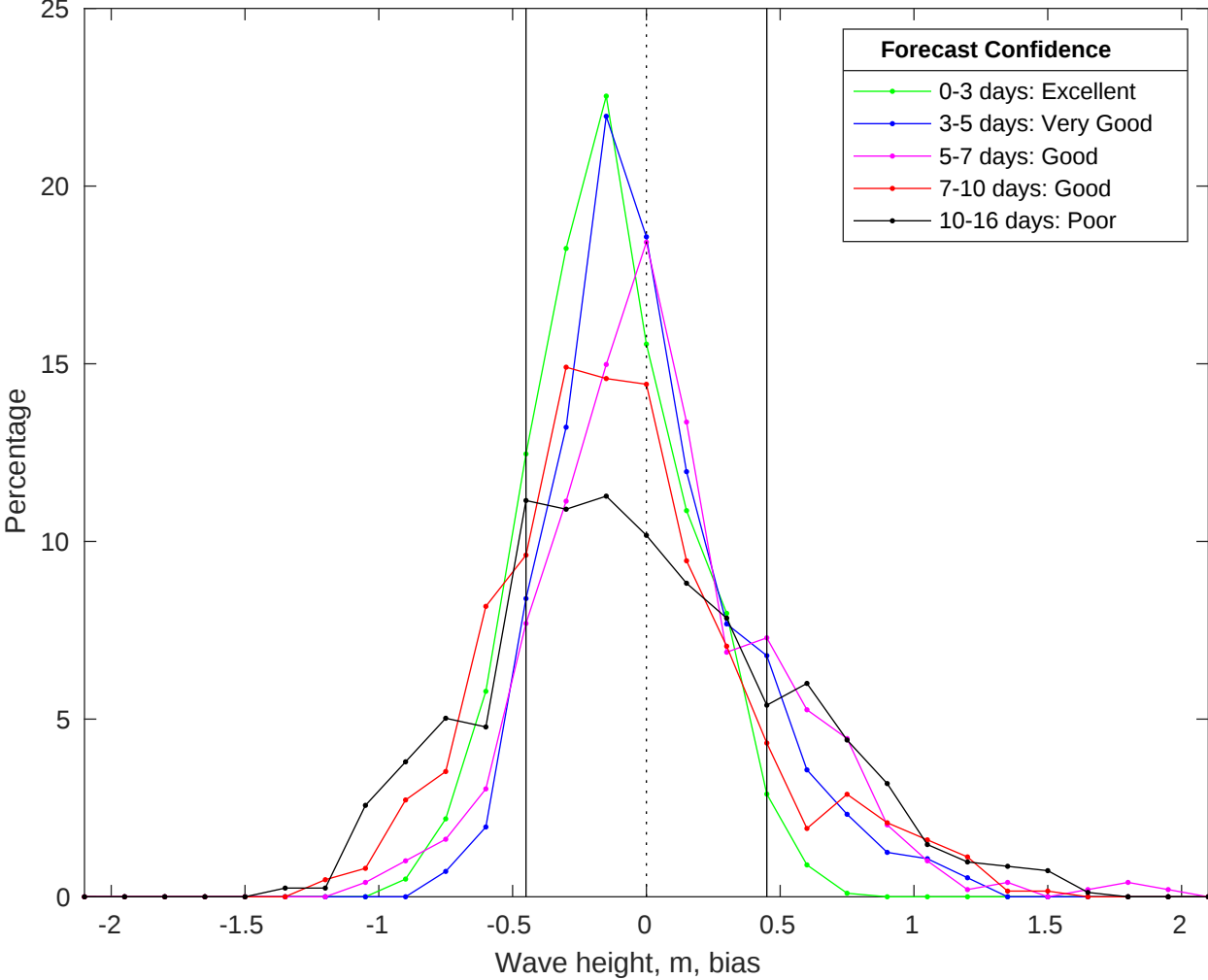
NDBC 46028 vs GFS Waves Bias Histogram: 17-Jul-2025
