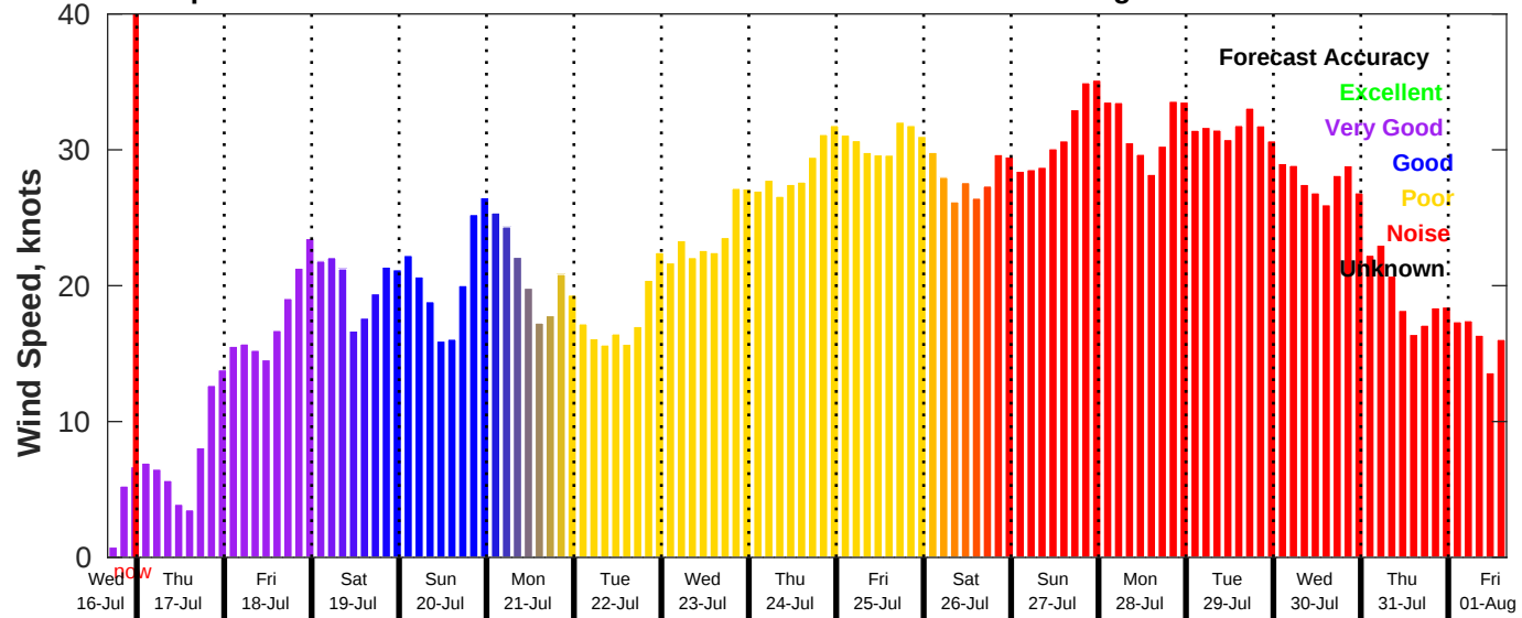
GFS Wind Speed Forecast for NDBC 46028 from 16-Jul-2025 16:00:00 to 01-Aug-2025 16:00:00
