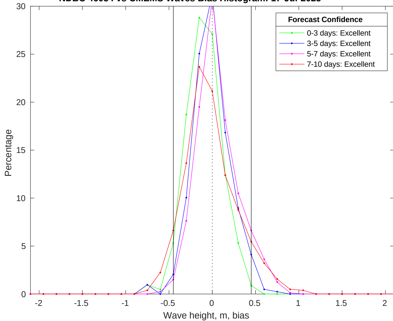
NDBC 46054 vs CMEMS Waves Bias Histogram: 17-Jul-2025
