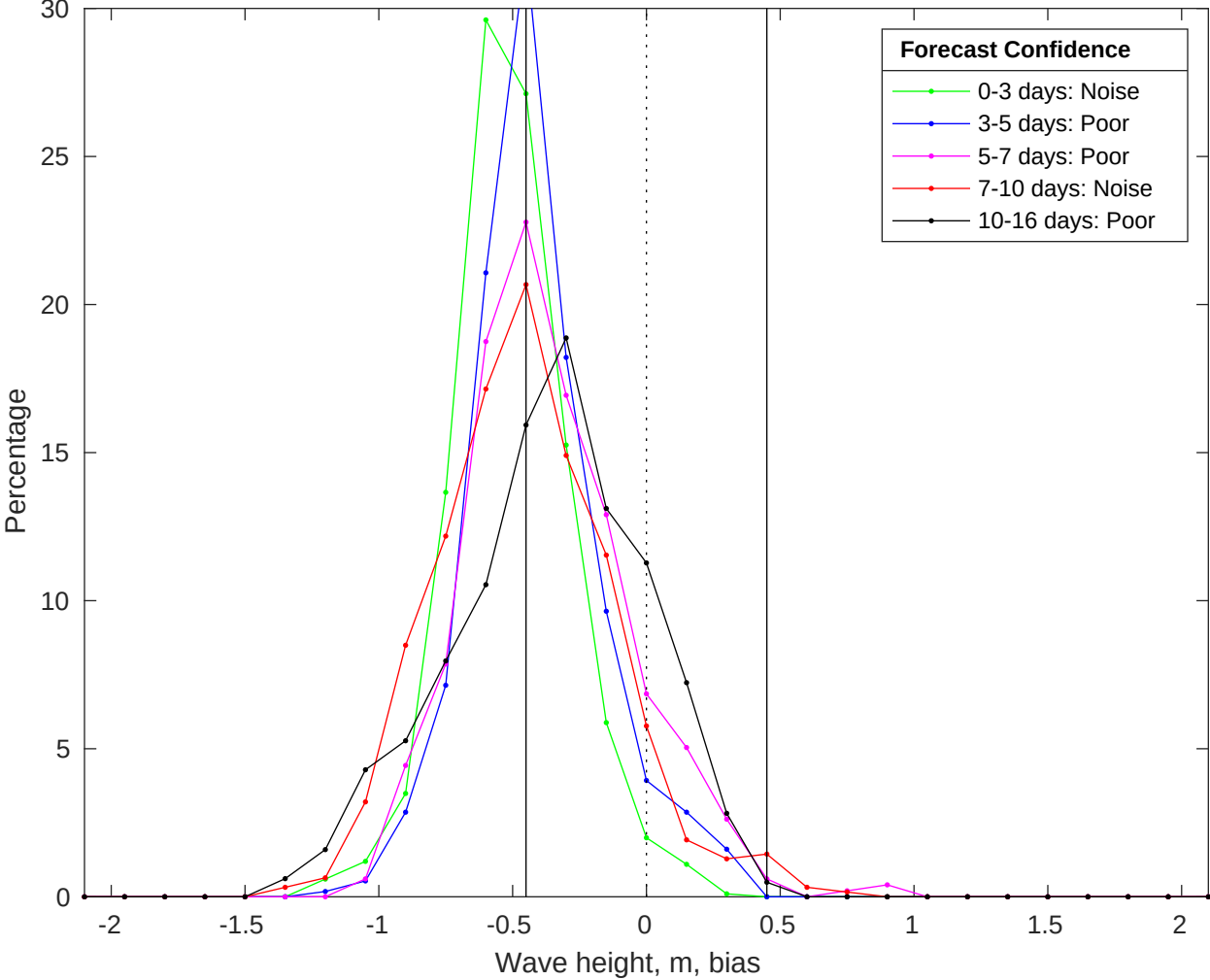
NDBC 46054 vs GFS Waves Bias Histogram: 17-Jul-2025
