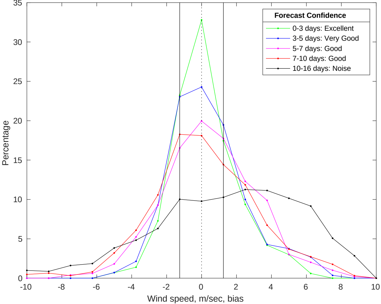
NDBC 46054 vs GFS Winds Bias Histogram: 17-Jul-2025
