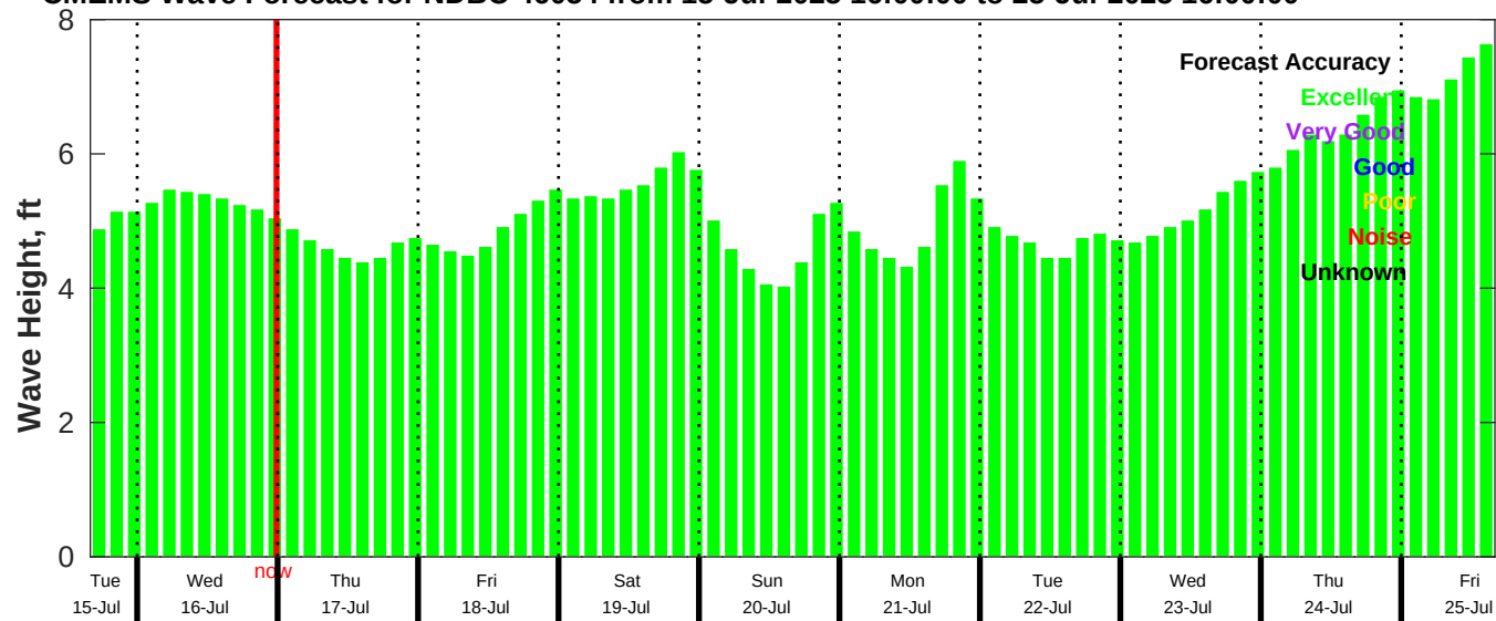
CMEMS Wave Forecast for NDBC 46054 from 15-Jul-2025 16:00:00 to 25-Jul-2025 16:00:00
