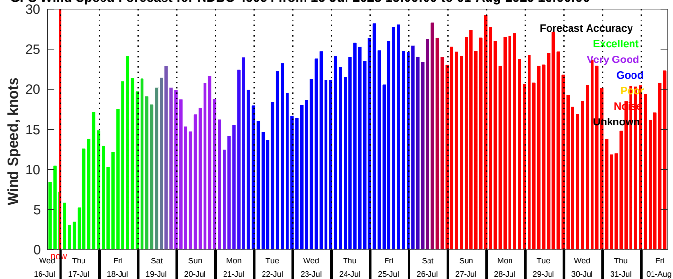
GFS Wind Speed Forecast for NDBC 46054 from 16-Jul-2025 16:00:00 to 01-Aug-2025 16:00:00
