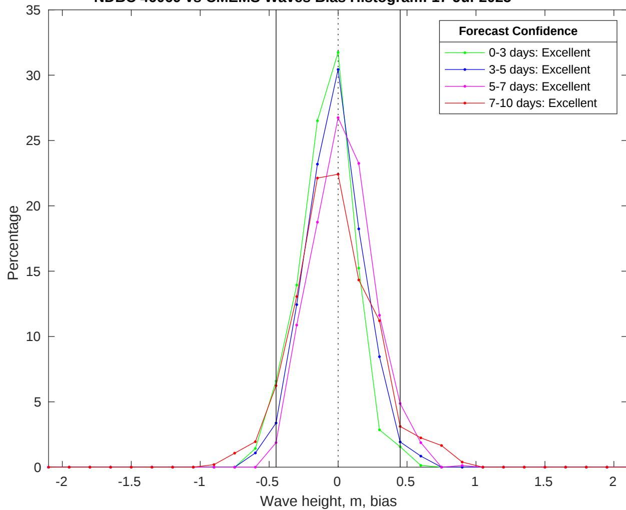
NDBC 46069 vs CMEMS Waves Bias Histogram: 17-Jul-2025
