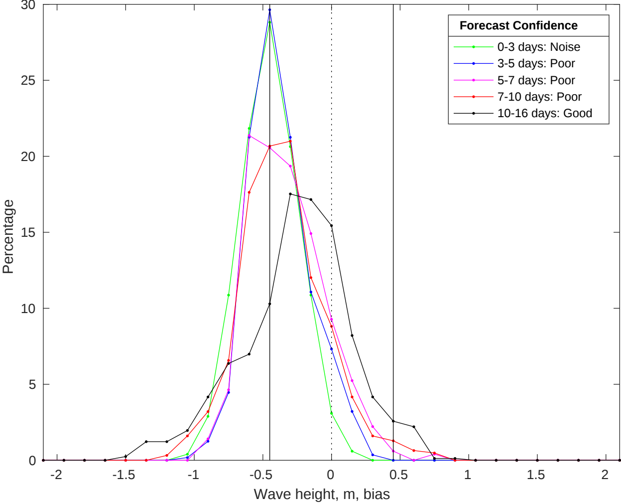
NDBC 46069 vs GFS Waves Bias Histogram: 17-Jul-2025
