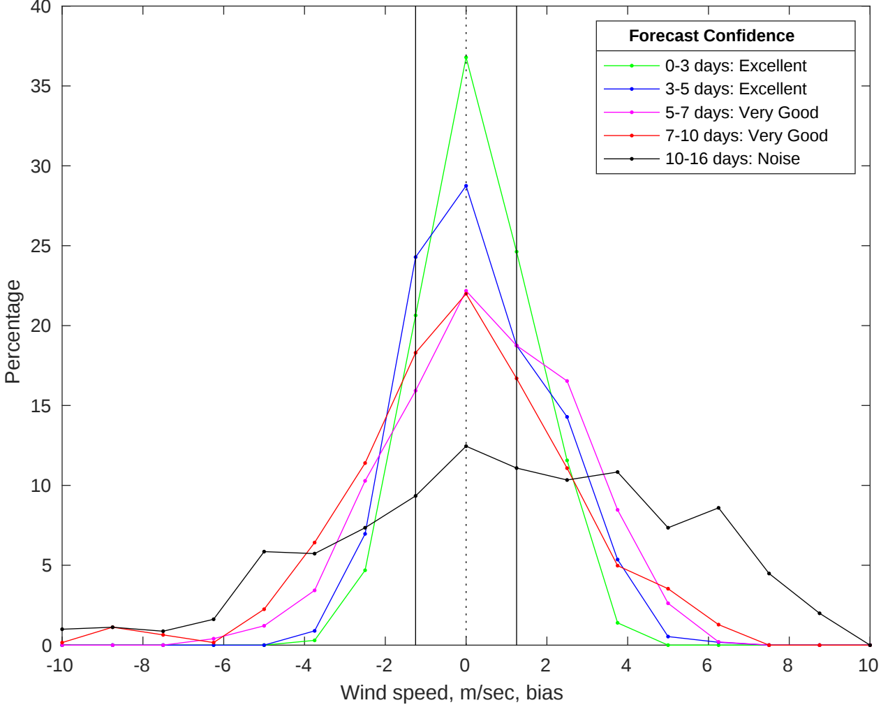
NDBC 46069 vs GFS Winds Bias Histogram: 17-Jul-2025
