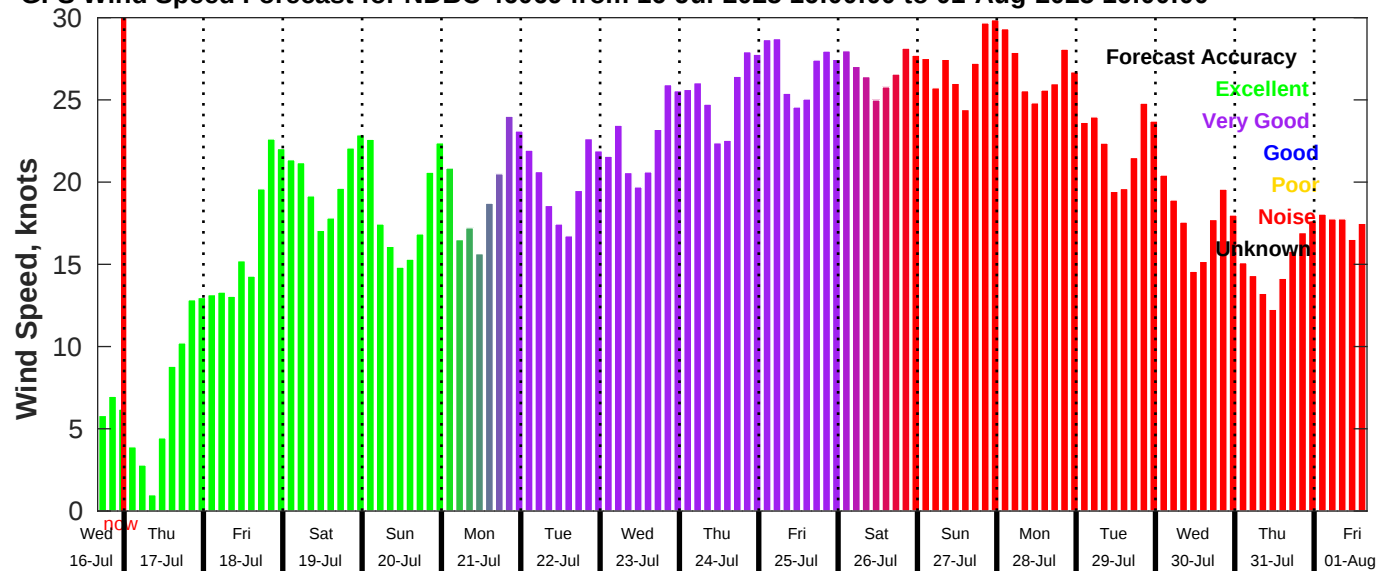
GFS Wind Speed Forecast for NDBC 46069 from 16-Jul-2025 16:00:00 to 01-Aug-2025 16:00:00
