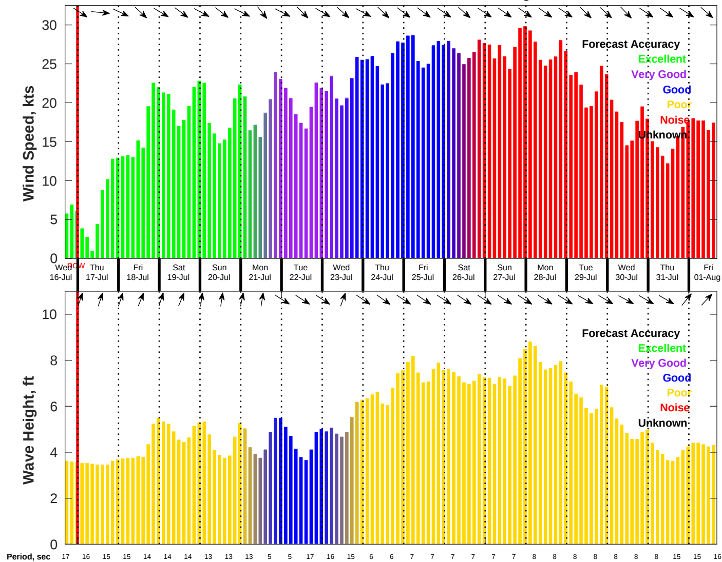
Wind & Wave Forecast for NDBC 46069 from 16-Jul-2025 16:00:00 to 01-Aug-2025 16:00:00
