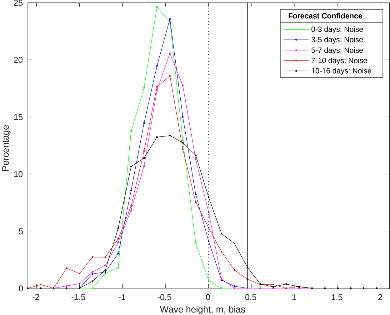
NDBC 51209 vs GFS Waves Bias Histogram: 17-Jul-2025
