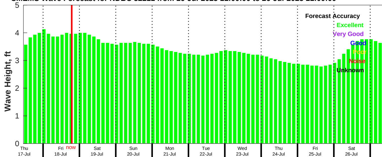
CMEMS Wave Forecast for NDBC 52211 from 16-Jul-2025 11:00:00 to 26-Jul-2025 11:00:00
