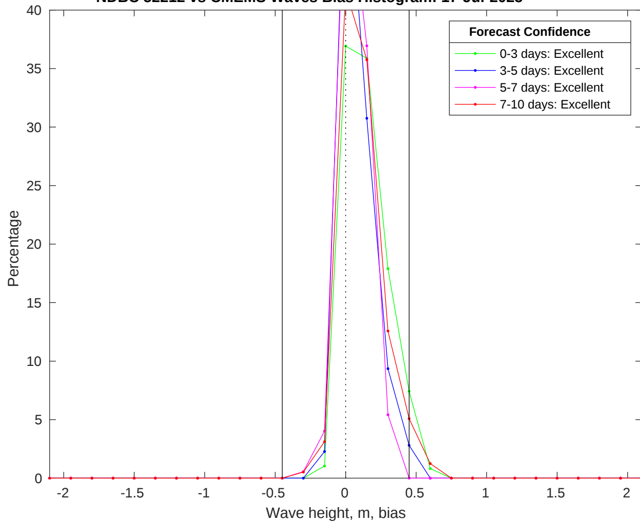
NDBC 52212 vs CMEMS Waves Bias Histogram: 17-Jul-2025
