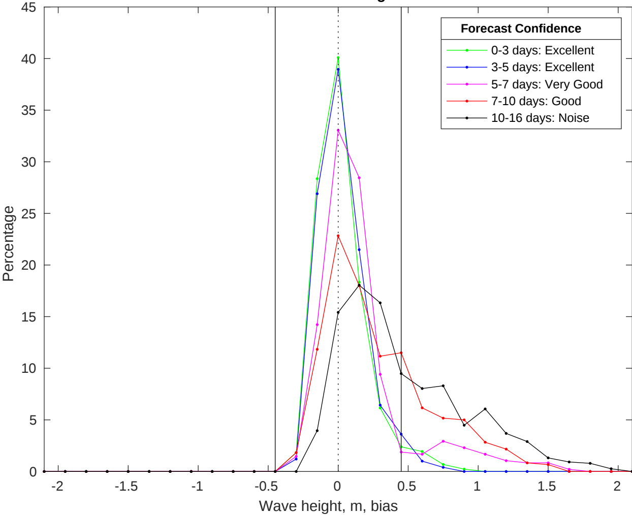
NDBC 52212 vs GFS Waves Bias Histogram: 17-Jul-2025
