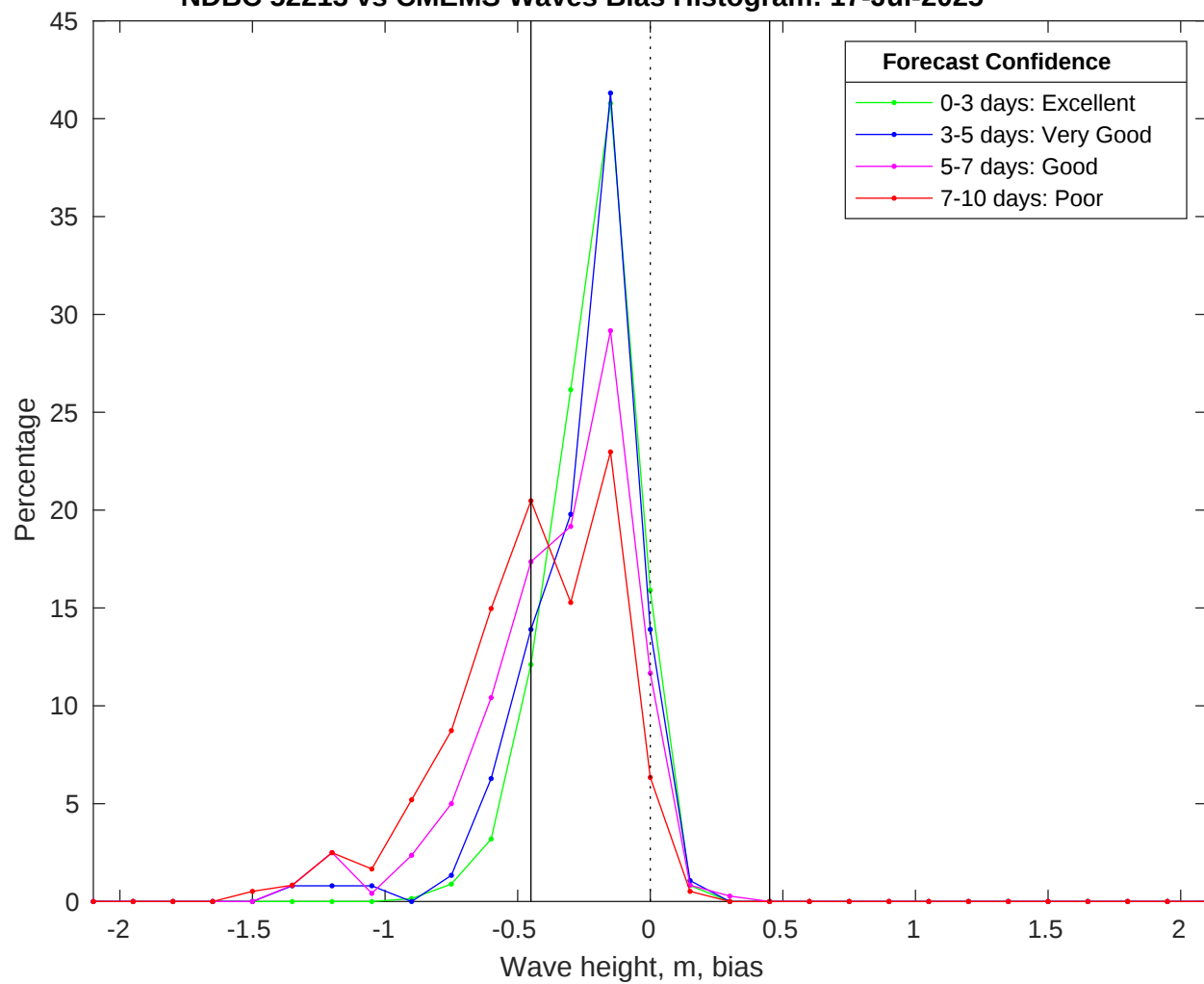
NDBC 52213 vs CMEMS Waves Bias Histogram: 17-Jul-2025
