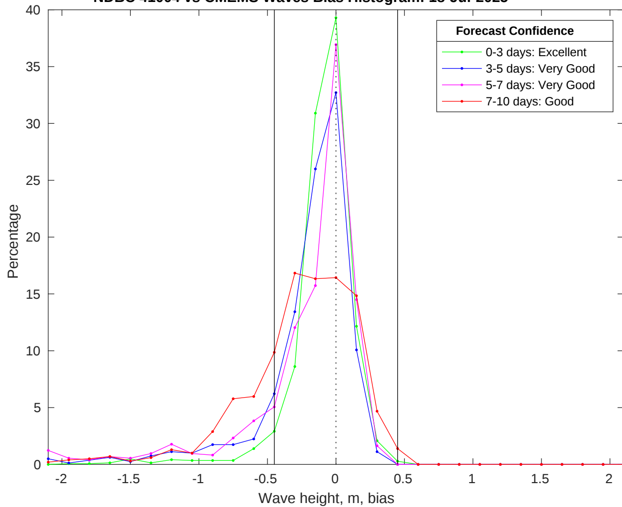
NDBC 41004 vs CMEMS Waves Bias Histogram: 18-Jul-2025
