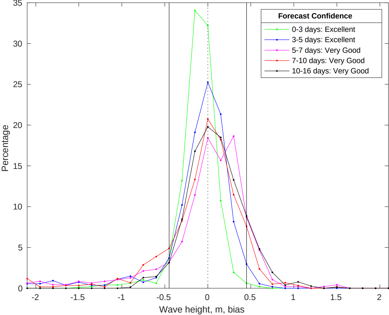
NDBC 41004 vs GFS Waves Bias Histogram: 18-Jul-2025
