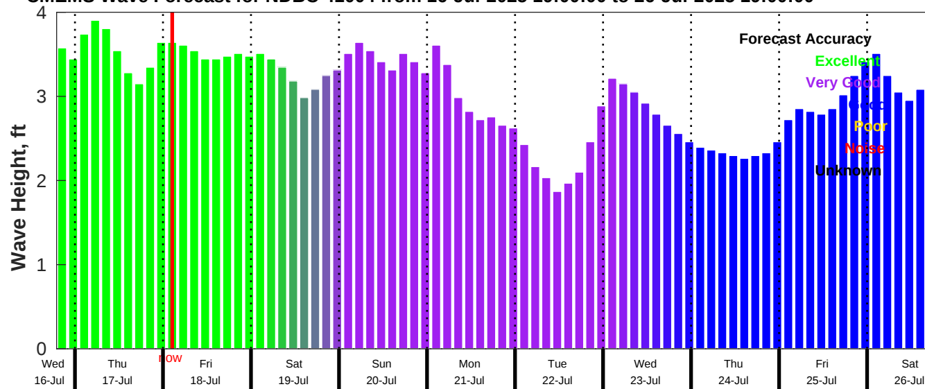
CMEMS Wave Forecast for NDBC 41004 from 16-Jul-2025 19:00:00 to 26-Jul-2025 19:00:00
