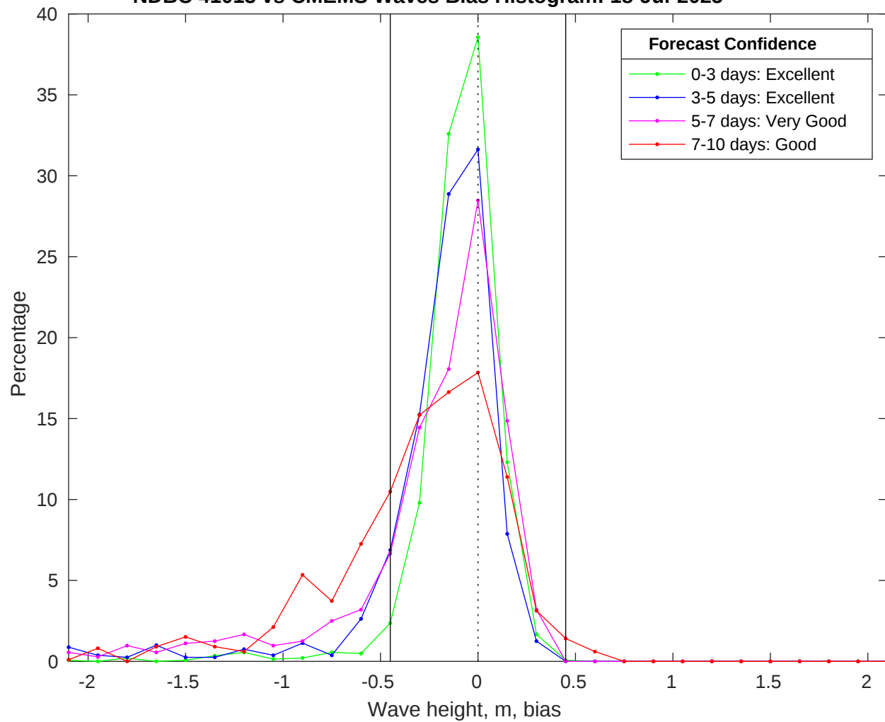
NDBC 41013 vs CMEMS Waves Bias Histogram: 18-Jul-2025
