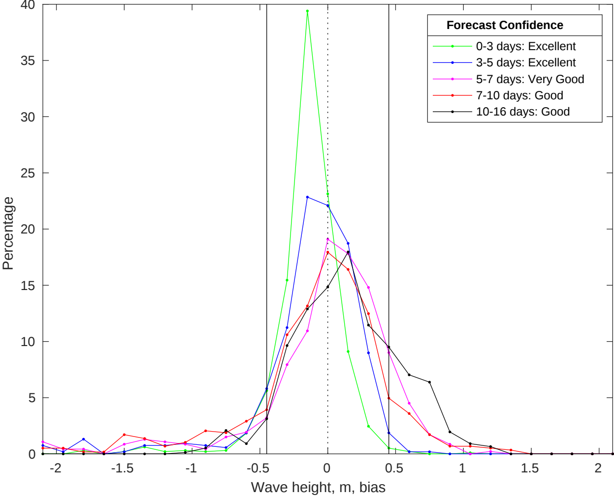
NDBC 41013 vs GFS Waves Bias Histogram: 18-Jul-2025
