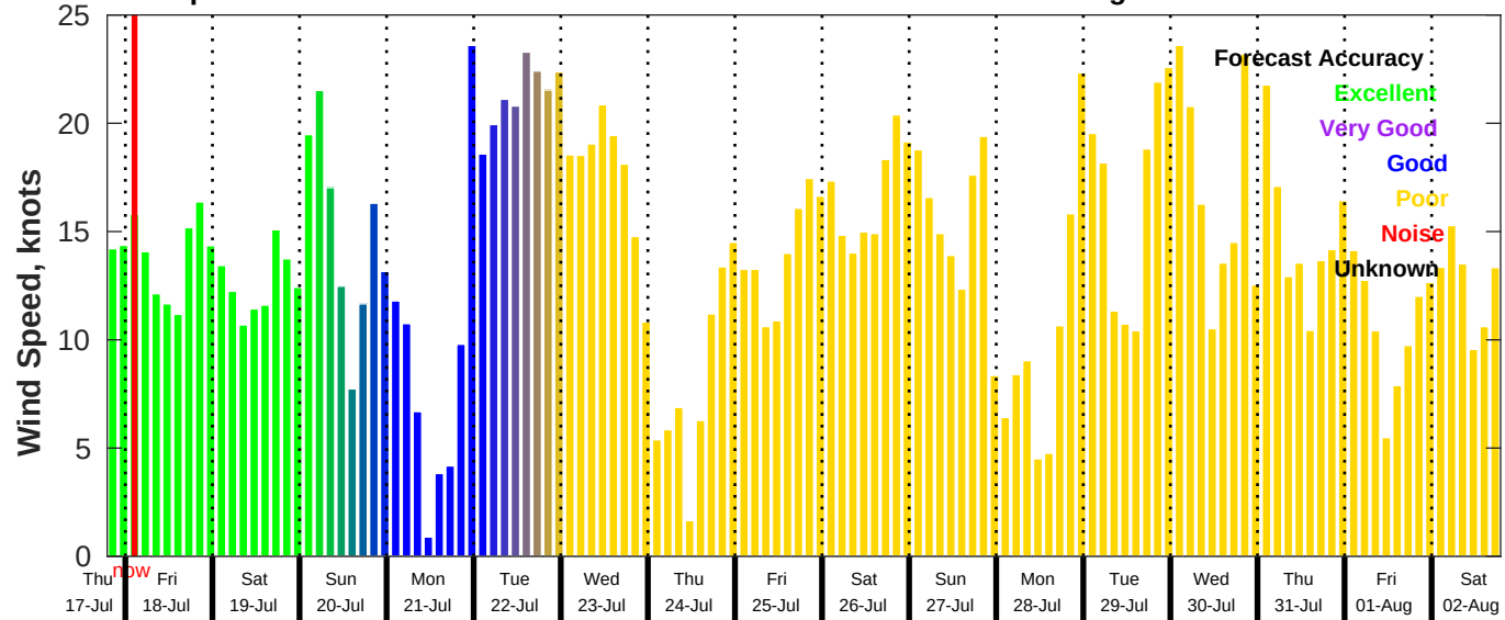
GFS Wind Speed Forecast for NDBC 41013 from 17-Jul-2025 19:00:00 to 02-Aug-2025 19:00:00
