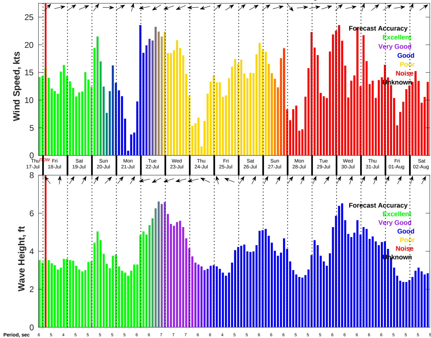
Wind & Wave Forecast for NDBC 41013 from 17-Jul-2025 19:00:00 to 02-Aug-2025 19:00:00
