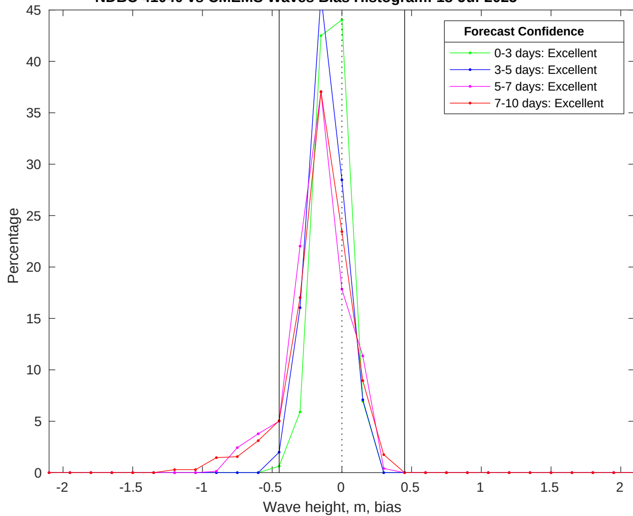
NDBC 41040 vs CMEMS Waves Bias Histogram: 18-Jul-2025
