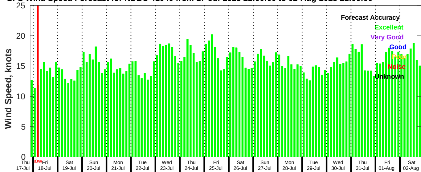
GFS Wind Speed Forecast for NDBC 41040 from 17-Jul-2025 21:00:00 to 02-Aug-2025 21:00:00
