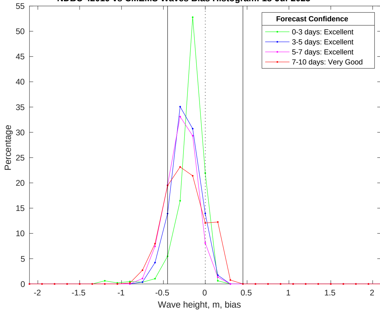
NDBC 42019 vs CMEMS Waves Bias Histogram: 18-Jul-2025
