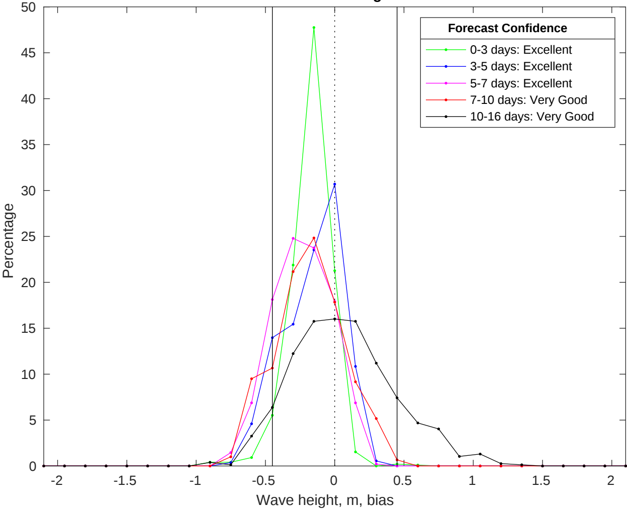
NDBC 42019 vs GFS Waves Bias Histogram: 18-Jul-2025
