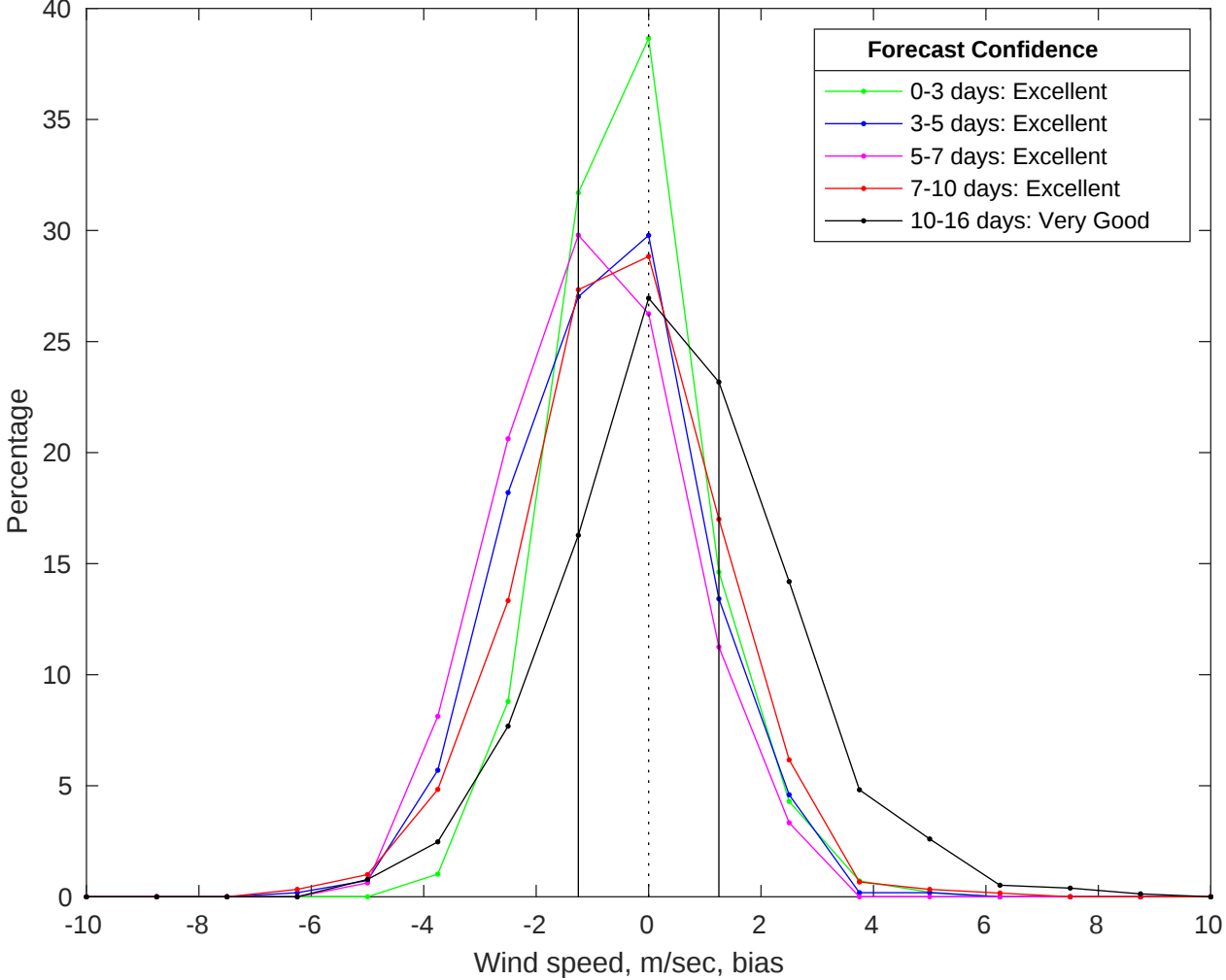
NDBC 42019 vs GFS Winds Bias Histogram: 18-Jul-2025
