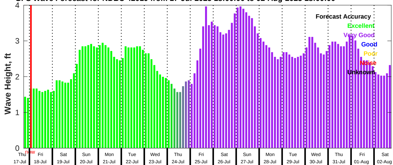
GFS Wave Forecast for NDBC 42019 from 17-Jul-2025 18:00:00 to 02-Aug-2025 18:00:00
